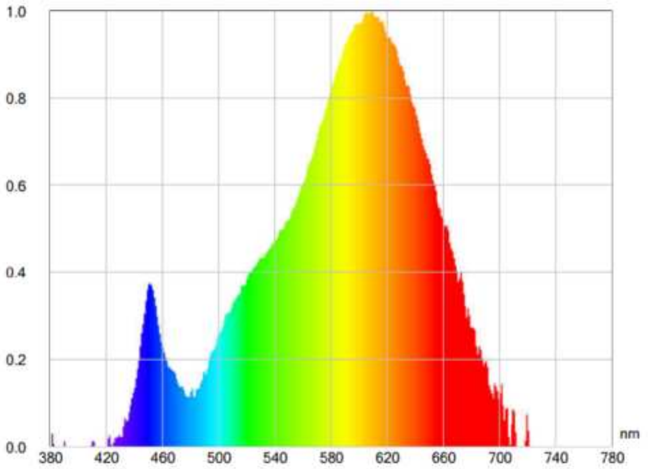
Spectrum Curve
