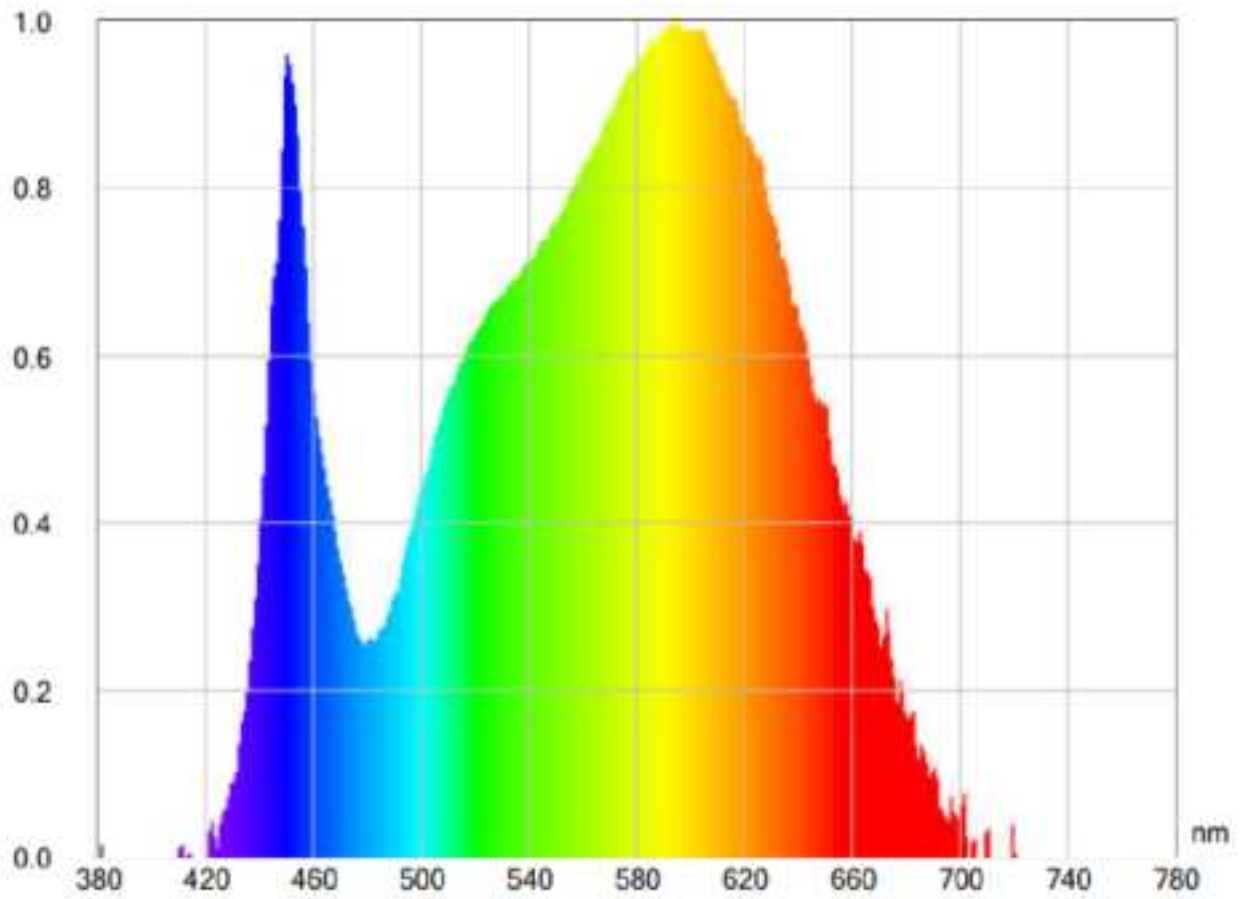
Spectrum Curve
